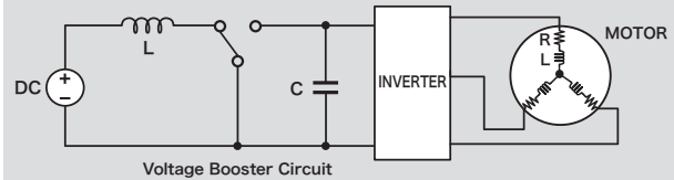
Voltage Booster Circuit
